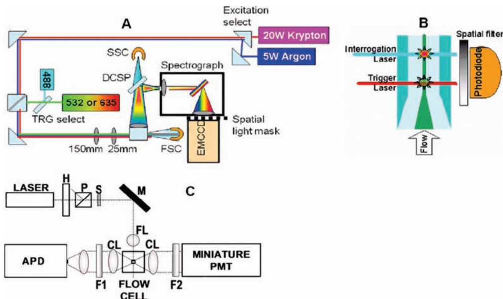
Figure 1. (a) Top-view schematic of Raman full-spectral flow cytometer experimental apparatus with grating-spectrograph dispersive element. Flip mirrors are used to allow selection of krypton or argon laser excitation and 488 nm or diode laser (532 or 635 nm) for the trigger (TRG) laser. DCSP: dichroic short pass filter, SSC: side scatter PMT detector, FSC: forward scatter photodiode detector. (b) Side-view schematic of flow cell showing spatial separation of trigger and interrogation lasers. Sample stream (dark central region) is hydrodynamically focused by the surrounding sheath flow (lighter colored region). (c) Diagram of the high-sensitivity cytometer optics breadboard, flow cell, and sample holder. H, half wave plate; P, polarizer; S, shutter; M, mirror; FL, focusing lens; CL, collection lens; F1, filter 1; F2, filter 2; PMT photomultiplier tube and APD avalanche photodiode.
