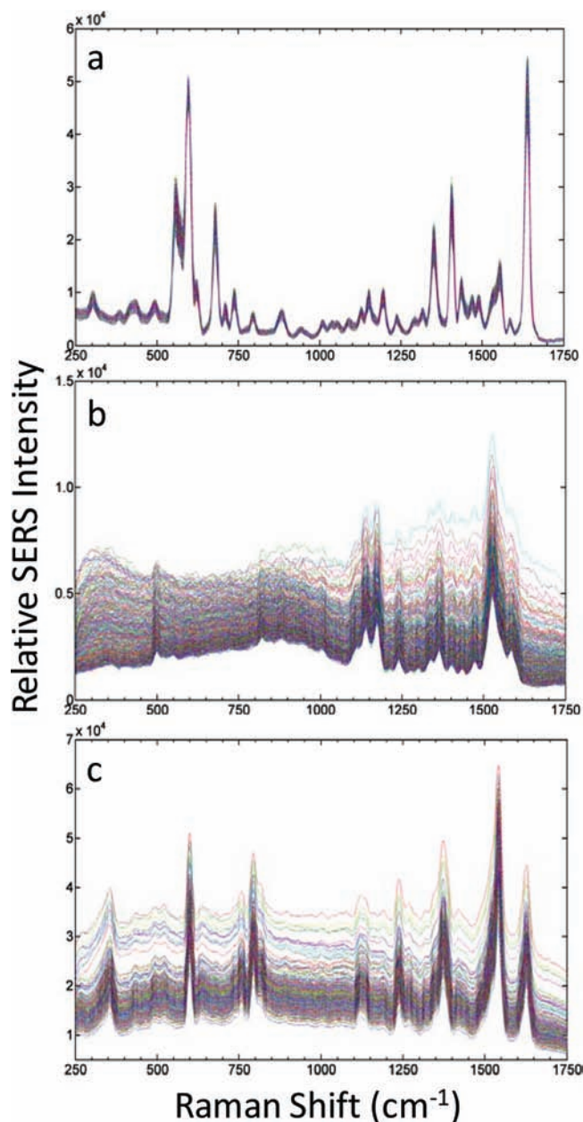
Figure 3. Plot of spectra from 1000 single SERS-tags, taken with 50 mW of 514 nm excitation from: (a) Oxazine 170 tags; (b) Styryl 9 M tags; (c) safranine tags (with 50 mW of 488 nm excitation). Integration time of 20 \mu s for each spectrum. A background spectrum from PBS has been subtracted from each single-tag spectrum.
