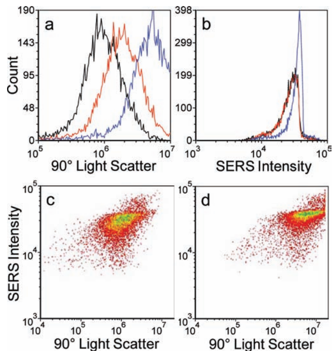
Figure 8. Univariate histograms of: (a) Side scatter intensity; and (b) SERS intensity for approximately 8,000 safranine-labeled SERS-tags as a function of three different laser power levels: 1 mW (black), 1.5 mW (red), 3 mW (blue). For comparison, bivariate histograms for the same particle sets showing light scatter versus Raman signal for: (c) 1 mW laser power; (d) 3 mW laser power. Excitation at 532 nm, 250 \mu s integration time per particle. Color contours represent particle counts as per Figure 6.
