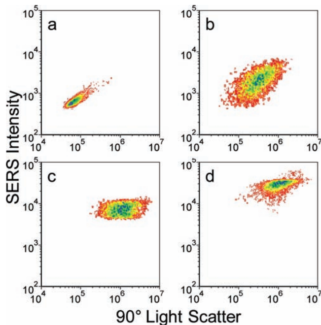
Figure 6. Bivariate histograms of (a) \sim 100 nm beads and (b–d) silver nanoparticle aggregates. Each histogram represents roughly 10,000 individual particles. Color contours represent particle counts, with red corresponding to fewer/individual particles and blue corresponding to greatest number of particles. (a) 100 nm fluorescent microspheres. (b) Oxazine 170. (c) Styryl 9M. (d) Safranin. Samples were interrogated at 532 nm, with 1 mW of power, and 250 \mu s integration time per particle.
