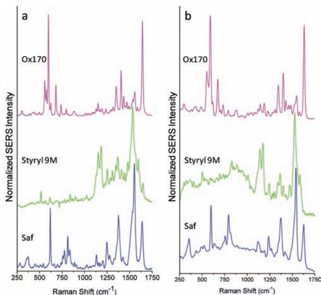
Figure 2. (a) Bulk spectra of oxazine 170 (Ox170), styryl 9 M and safranin (Saf) SERS-tags taken with 0.5 mW of 514 or 488 nm (safranin only) excitation, 10 s integration times. (b) Analogous spectra taken in flow on a single SERS-tag particle with 50 mW of 514 or 488 nm (safranin only) excitation, 20 \mu\text{s} integration times.
